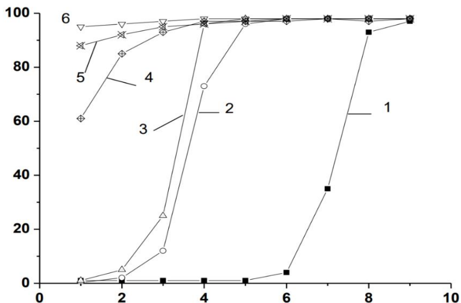
Figure 2. Diagram of the kinetic state of cyanide loss during airborne driving of HCN in MBA (1) and bubble column (2)
